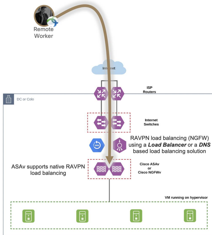
Figure 16: Remote access VPN termination on ASAv and NGFWv (HA, and VPN Load Balancing)
