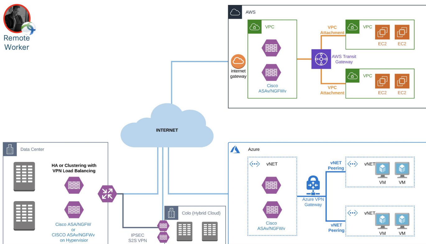
Figure 6: Remote worker in a multi-cloud environment
