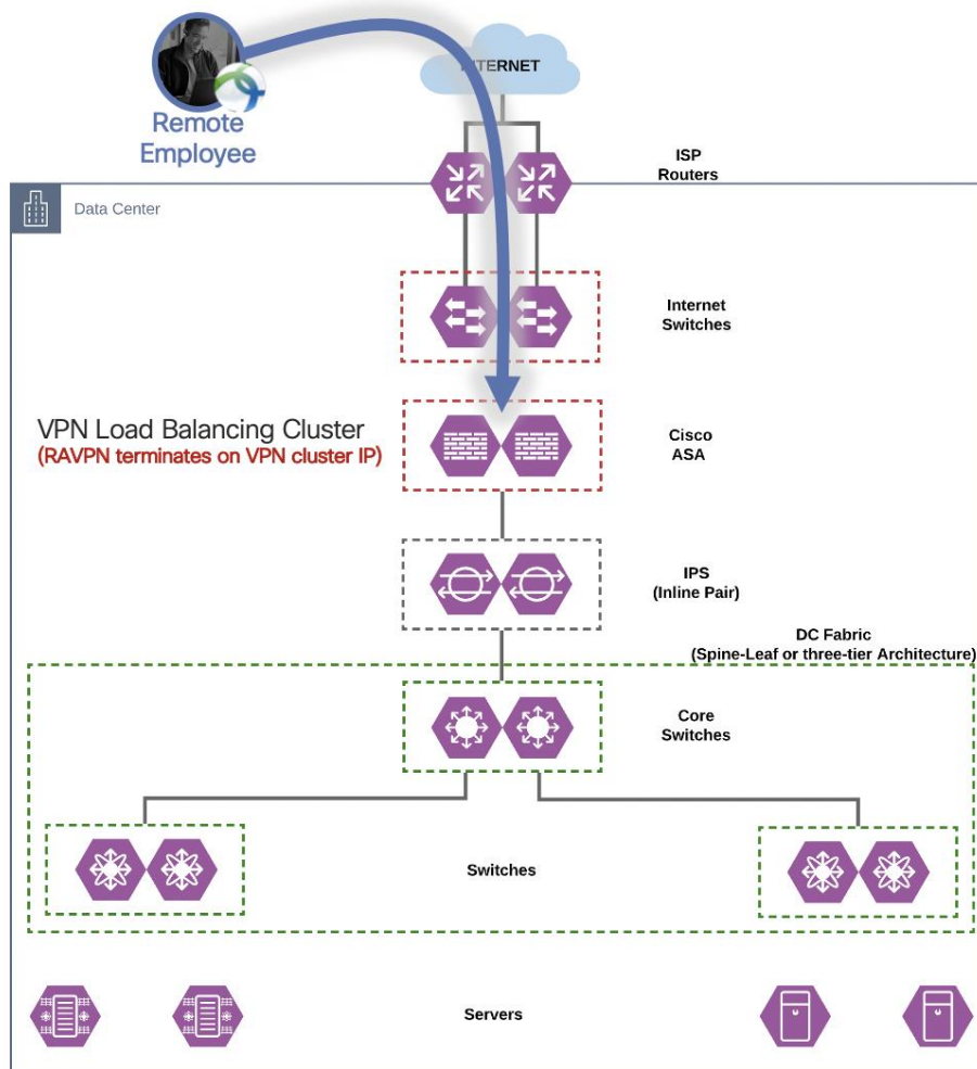
Figure 14: Remote access VPN termination on ASA (native VPN load balancing)
