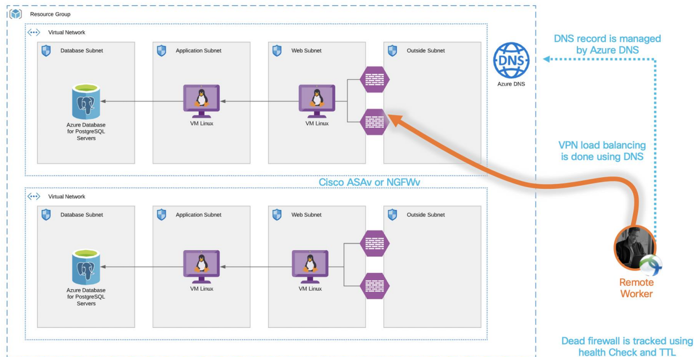
Figure 18: DNS based remote access VPN load balancing in Azure
