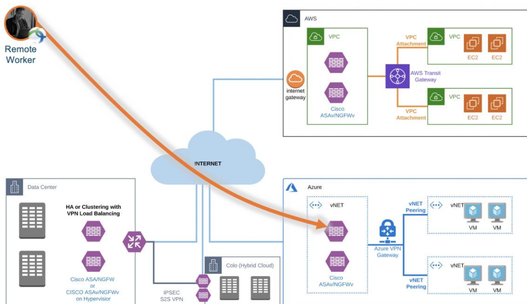
Figure 13: Remote access VPN termination on firewalls deployed in Azure
