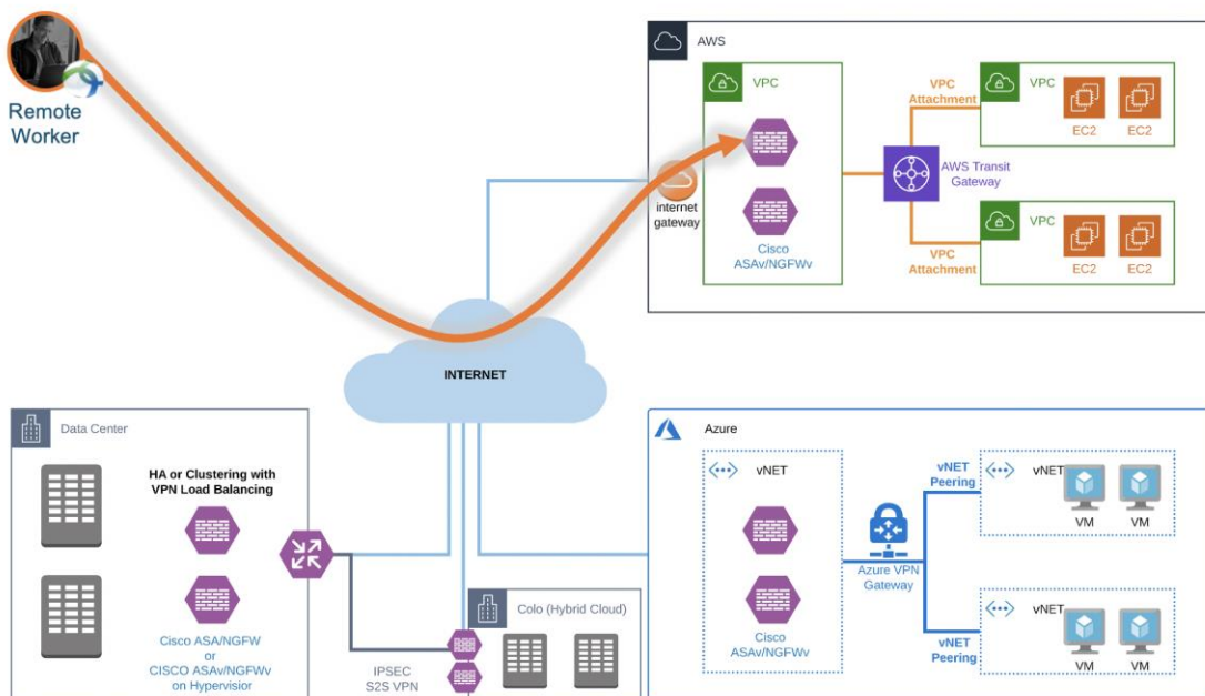
Figure 12: Remote access VPN termination on firewalls deployed in AWS
