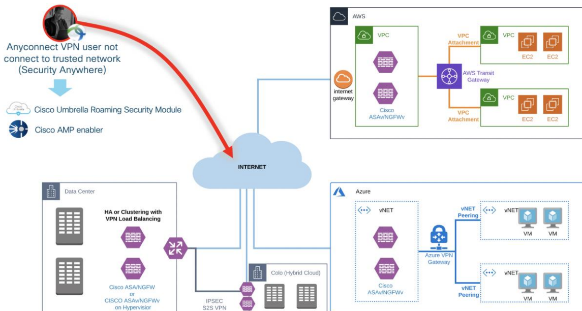
Figure 8: Remote worker on internet
