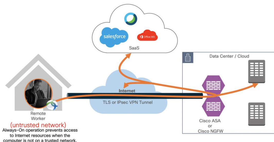
Figure 22: VPN always-on feature
