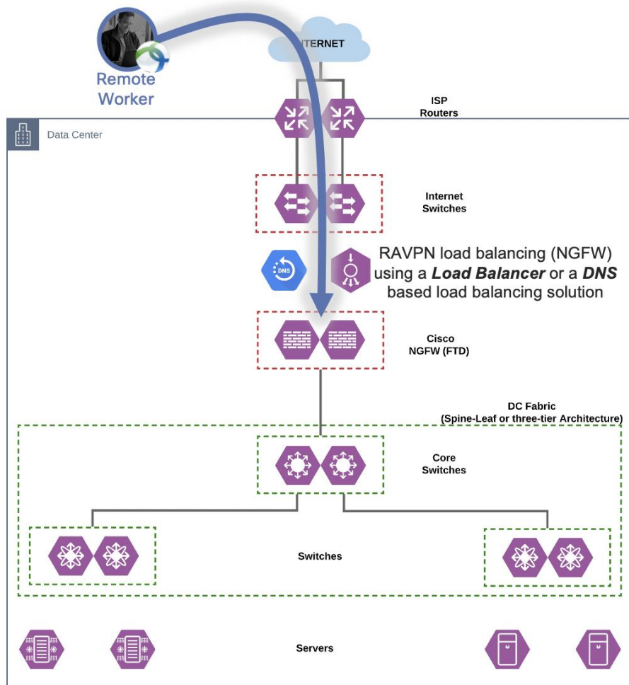
Figure 15: Remote access VPN termination on NGFW (HA, and VPN load balancing using LB or DNS)
