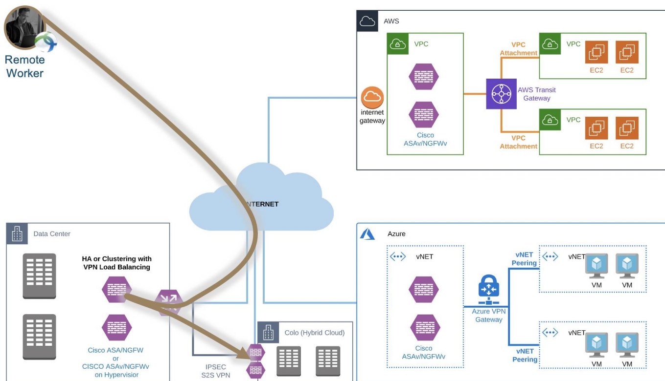
Figure 10: Remote worker accessing Colo resources via Data Center firewall
