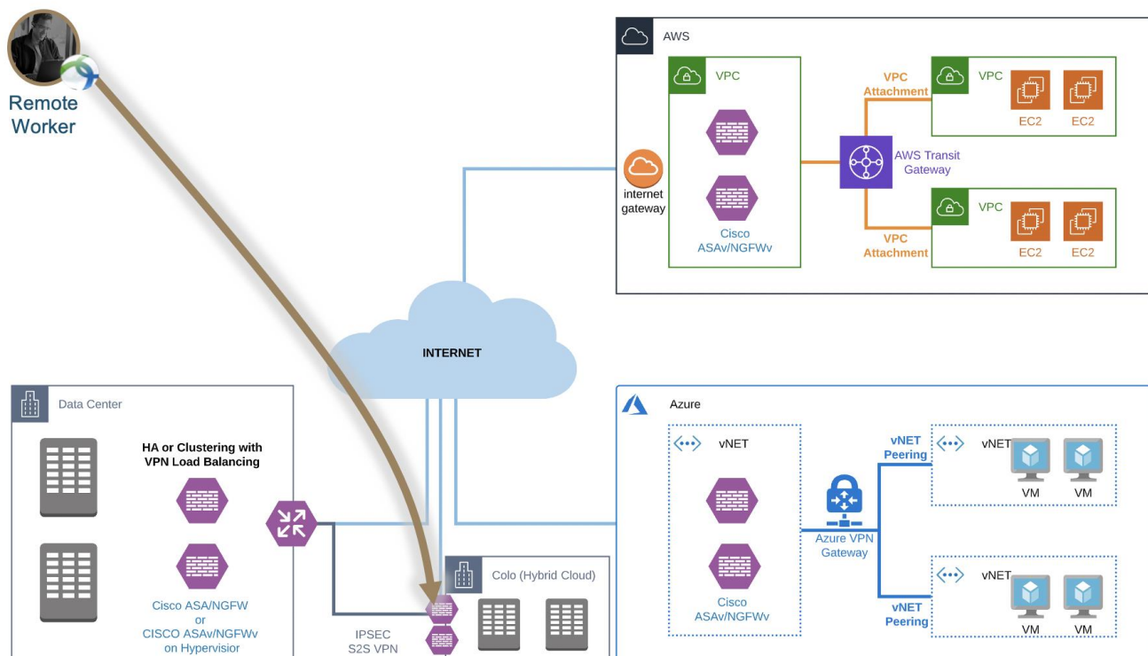
Figure 11: Remote worker connected to Colo firewalls
